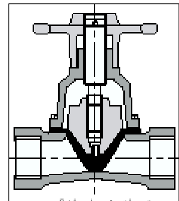
CAST IRON DIAPHRAGM VALVE
